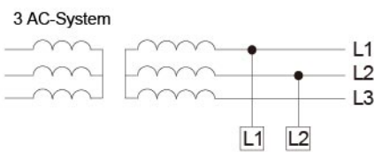
Connection to the 3AC system
